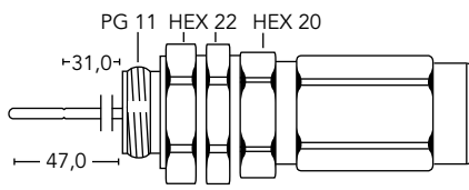
PG11mu-XX
