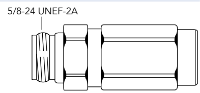
Nf-XX
