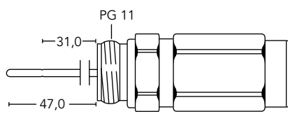
PG11m-XX
